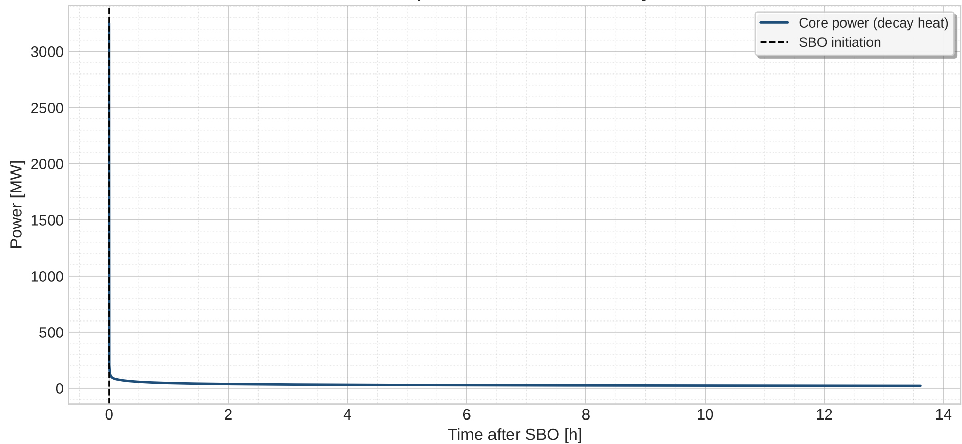
No SG Depressurization - Core Decay Heat
